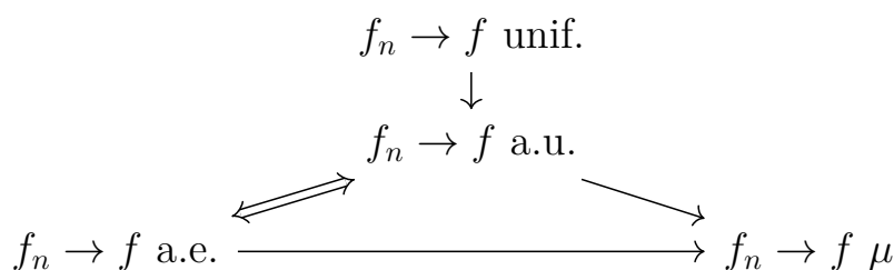
Figure 4.1: In a finite measure space
