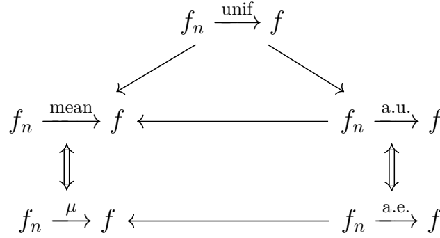
Figure 4.2: there exists g \in \mathcal{L}^1(\mu) such that |f_n| \leq g for all n .
